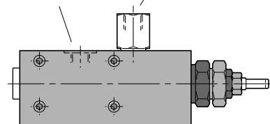
VP1-095/-130 control valve ports.
