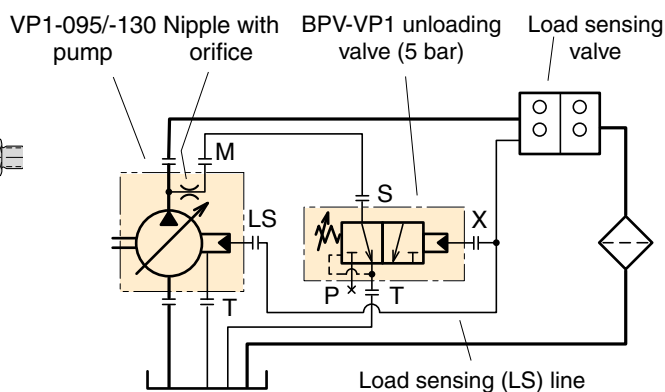
BPV-VP1 installation schematic with VP1-095/-130 pump.
